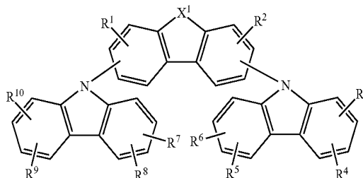
[Chemical Formula 1]
