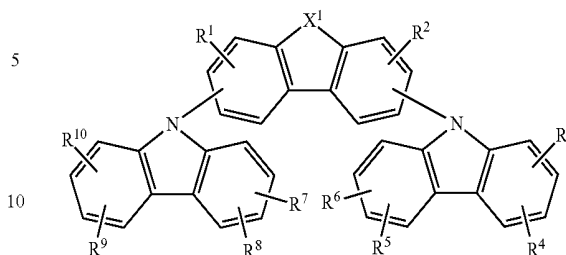
[Chemical Formula 1]
