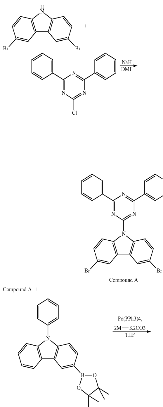
[Reaction Scheme 1]
