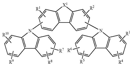
[Chemical Formula 1]
