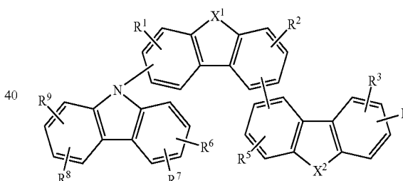
[Chemical Formula 2]
